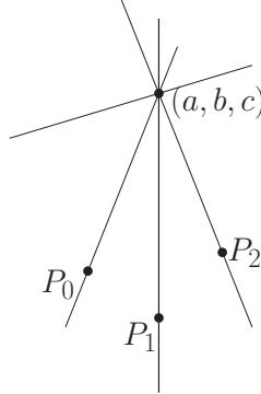
FIGURE 1. Quartic with a quadruple point
